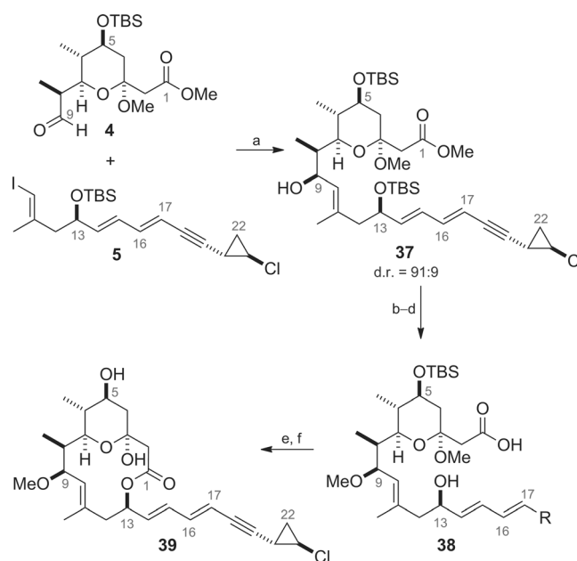
Scheme 4. Reagents and conditions: a) i) 5 , (1.3 equiv), t BuLi, Et 2 O, -78 °C; ii) ZnBr 2 , Et 2 O, -78 → 0 °C; iii) (1 S ,2 R )-(+)- N -methylephedrine (1.1 equiv), n BuLi, PhMe, 0 °C; iv) 4 , PhMe, 0 °C, 48%; b) MeOTf, DTBP, CH 2 Cl 2 , RT, 73%; c) TBAF, THF, RT, 74%; d) Ba(OH) 2 ·8 H 2 O, MeOH, RT, quant.; e) 2,4,6-trichlorobenzoyl chloride, Et 3 N, RT, then addition to DMAP, PhMe, 80 °C; f) TFA, THF/H 2 O (5:1), RT, 58% over 2 steps. DTBP = 2,6-di- tert -butylpyridine; TFA = trifluoroacetic acid.
