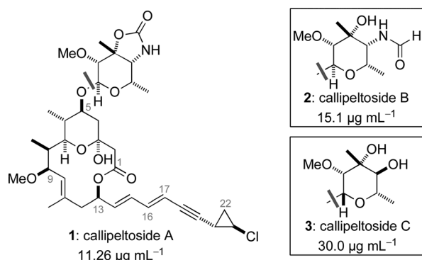
Figure 1. The callipeltoside family of natural products and corresponding IC 50 values against the NSCLC-N6 cell line.
