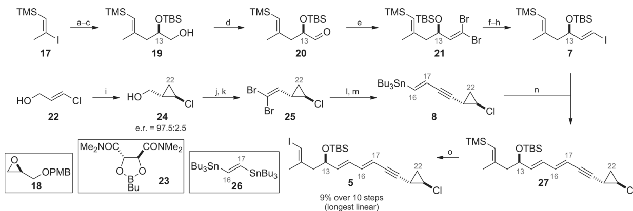
Scheme 2. Reagents and conditions: a) t BuLi, PhMe, -78^{\circ}\text{C} , then 18 , \text{BF}_3\cdot\text{OEt}_2 , PhMe; b) TBSOTf, 2,6-lutidine, \text{CH}_2\text{Cl}_2 , -78^{\circ}\text{C} , 53% over 2 steps; c) DDQ, pH 7 phosphate buffer, \text{CH}_2\text{Cl}_2 , 0^{\circ}\text{C} , 89%; d) \text{SO}_3\cdot\text{Py} , \text{Et}_3\text{N} , DMSO, \text{CH}_2\text{Cl}_2 , 0^{\circ}\text{C}\rightarrow\text{RT} ; e) \text{PPh}_3 , \text{CBr}_4 , \text{CH}_2\text{Cl}_2 , then 20 , 2,6-lutidine, \text{CH}_2\text{Cl}_2 , 0^{\circ}\text{C} , 89% over 2 steps; f) n BuLi, THF, -78^{\circ}\text{C} , then \text{H}_2\text{O} , 85%; g) \text{Pd}(\text{PPh}_3)_2\text{Cl}_2 (3 mol%), \text{Bu}_3\text{SnH} , THF, 0^{\circ}\text{C} ; h) \text{I}_2 , \text{CH}_2\text{Cl}_2 , -78^{\circ}\text{C} , 49% over 2 steps; i) \text{ZnEt}_2 , \text{CH}_2\text{Cl}_2 , 0^{\circ}\text{C} , then 23 , \text{CH}_2\text{Cl}_2 , 0^{\circ}\text{C}\rightarrow\text{RT} , 74%; j) PCC, celite, \text{CH}_2\text{Cl}_2 , RT; k) \text{PPh}_3 , \text{CBr}_4 , \text{CH}_2\text{Cl}_2 , 0^{\circ}\text{C} , then aldehyde, \text{CH}_2\text{Cl}_2 , 0^{\circ}\text{C}\rightarrow\text{RT} , 70% over 2 steps; l) TBAF, DMF, 65^{\circ}\text{C} ; m) \text{Pd}_2\text{dba}_3 (10 mol%), \text{AsPh}_3 (40 mol%), \text{Ag}_2\text{CO}_3 (1.0 equiv), THF, dark, -10^{\circ}\text{C} , then 26 , 45% over 2 steps; n) \text{Pd}(\text{PFur}_3)_2\text{Cl}_2 (15 mol%), DMF, dark, RT, 63%; o) NIS, MeCN, RT, 84%. DDQ = 2,3-dichloro-5,6-dicyano- p -benzoquinone; PCC = pyridinium chlorochromate; TBAF = tetrabutylammonium fluoride; NIS = N -iodosuccinimide.
