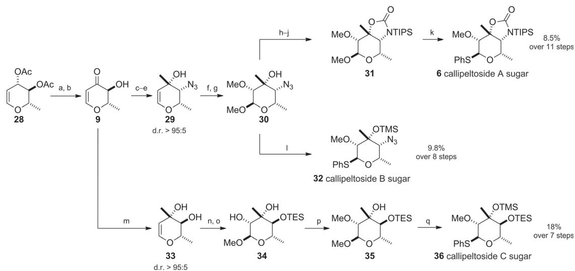
Scheme 3. Reagents and conditions: a) \text{PS}\cdot\text{Na}_2\text{CO}_3 , MeOH, RT; b) \text{MnO}_2 , \text{CH}_2\text{Cl}_2 , RT, 74% over 2 steps; c) \text{NaCl} , Py, \text{CH}_2\text{Cl}_2 , RT, 95%; d) n Bu 4 NN 3 , \text{CH}_2\text{Cl}_2 , 0^{\circ}\text{C} , 72%; e) MeLi, THF, -100^{\circ}\text{C} , 79%; f) m -CPBA, MeOH, 0^{\circ}\text{C}\rightarrow\text{RT} , 52%; g) \text{KOtBu} , MeI, THF, 0^{\circ}\text{C} , 79%; h) \text{H}_2 , \text{Pd}(\text{OH})_2 , EtOAc, RT, 93%; i) triphosgene, Py, THF, -78^{\circ}\text{C}\rightarrow\text{RT} , 72%; j) TIPSOTf, 2,6-lutidine, \text{CH}_2\text{Cl}_2 , RT, 97%; k) PhSH, \text{BF}_3\cdot\text{OEt}_2 , \text{CH}_2\text{Cl}_2 , 0^{\circ}\text{C}\rightarrow\text{RT} , 80%; l) \text{ZnI}_2 , TBAI, TMSSPh, DCE, 65^{\circ}\text{C} , 60%; m) MeLi-LiBr, \text{Et}_2\text{O} , -78^{\circ}\text{C} , 78%; n) TESCl, Py, DMAP, \text{CH}_2\text{Cl}_2 , RT; o) m -CPBA, MeOH, 0^{\circ}\text{C}\rightarrow\text{RT} , 45% over 2 steps; p) \text{KOtBu} , MeI, THF, 0^{\circ}\text{C} , 81%; q) \text{ZnI}_2 , TBAI, TMSSPh, DCE, 65^{\circ}\text{C} , 86%. \text{NaCl} = 4-nitrobenzenesulfonyl chloride; m -CPBA = 3-chloroperbenzoic acid; TIPS = triisopropylsilyl; TMS = trimethylsilyl; TES = triethylsilyl; DMAP = 4-( N,N -dimethylamino)pyridine; TBAI = tetrabutylammonium iodide.
