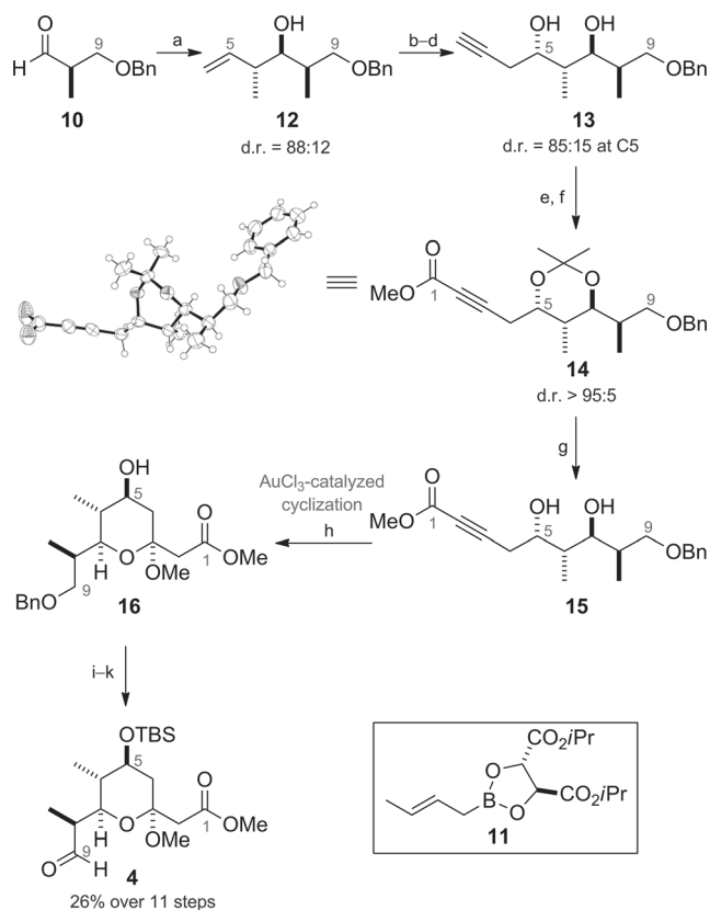
Scheme 1. Reagents and conditions: a) crotylborane 11 , 4 Å MS, PhMe, -78^{\circ}\text{C} , 70%; b) \text{OsO}_4 , NMO, acetone/ \text{H}_2\text{O} (2:1), RT; c) \text{NaIO}_4 , THF/ \text{H}_2\text{O} (10:1), 0^{\circ}\text{C} \rightarrow \text{RT} ; d) Zn, propargyl bromide, THF, 0 \rightarrow -100^{\circ}\text{C} , 72% over 3 steps; e) 2,2-dimethoxypropane, ( \pm )-CSA, acetone, RT; f) n BuLi, THF, -40 \rightarrow -78^{\circ}\text{C} , then \text{ClCO}_2\text{Me} , 73% over 2 steps; g) QP-SA, MeOH, RT, 95%; h) \text{AuCl}_3 (2 mol%), MeOH, RT, 96%; i) 2,6-lutidine, TBSOTf, \text{CH}_2\text{Cl}_2 , -78^{\circ}\text{C} , 91%; j) \text{H}_2 , Pd/C (10% wt), EtOAc, RT, 96%; k) Dess–Martin periodinane, \text{K}_2\text{CO}_3 , \text{CH}_2\text{Cl}_2 , RT, 87%. NMO = N -methylmorpholine N -oxide; ( \pm )-CSA = ( \pm )-camphor-sulfonic acid; QP-SA = Quadrapure sulfonic acid.
