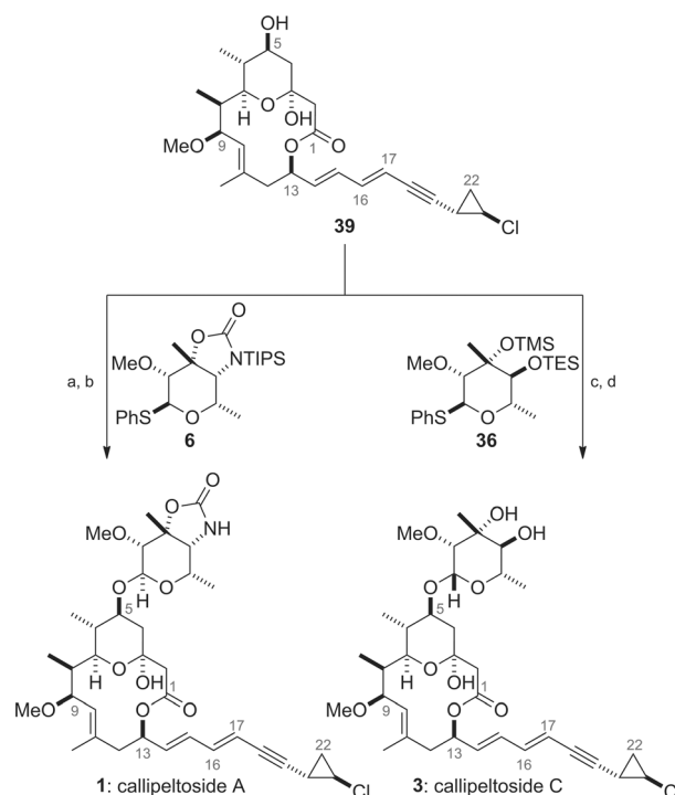
Scheme 5. Reagents and conditions: a) 39 , 6 , 4 Å MS, CH 2 Cl 2 , DTBMP, RT, 50 min, then -15 °C, NIS, TfOH, -15 °C → RT; b) TBAF, THF, 83% over 2 steps; c) 39 , 36 , 4 Å MS, CH 2 Cl 2 , DTBMP, RT, 50 min, then -15 °C, NIS, TfOH, -15 °C → RT; d) TASF, DMF, 40 °C, 57% over 2 steps. DTBMP = 2,6-di- tert -butyl-4-methylpyridine; TfOH = trifluoromethanesulfonic acid; TASF = tris(dimethylamino)sulfonium difluorotri-methylsilicate.
