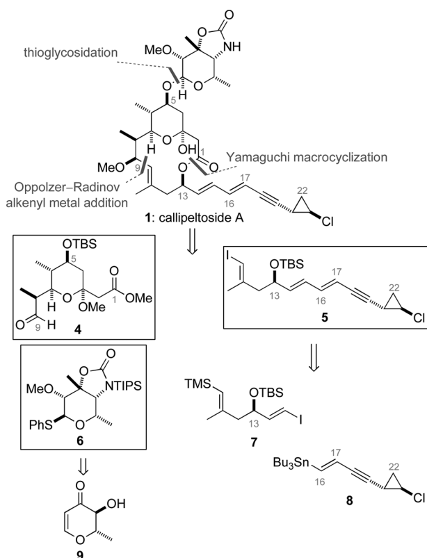
Figure 2. Retrosynthetic analysis of the callipeltoside family. Callipeltoside A shown for clarity.
